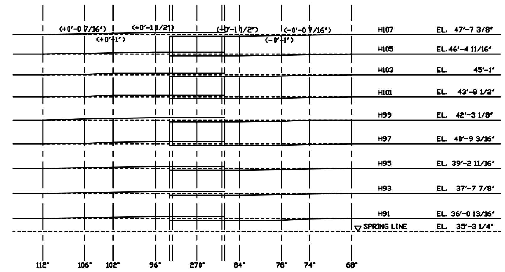
DOME HOOP No.1 S=1/15
