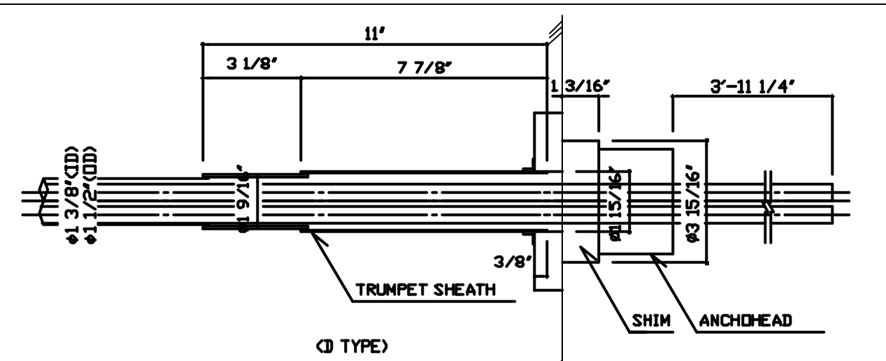
(D TYPE)
