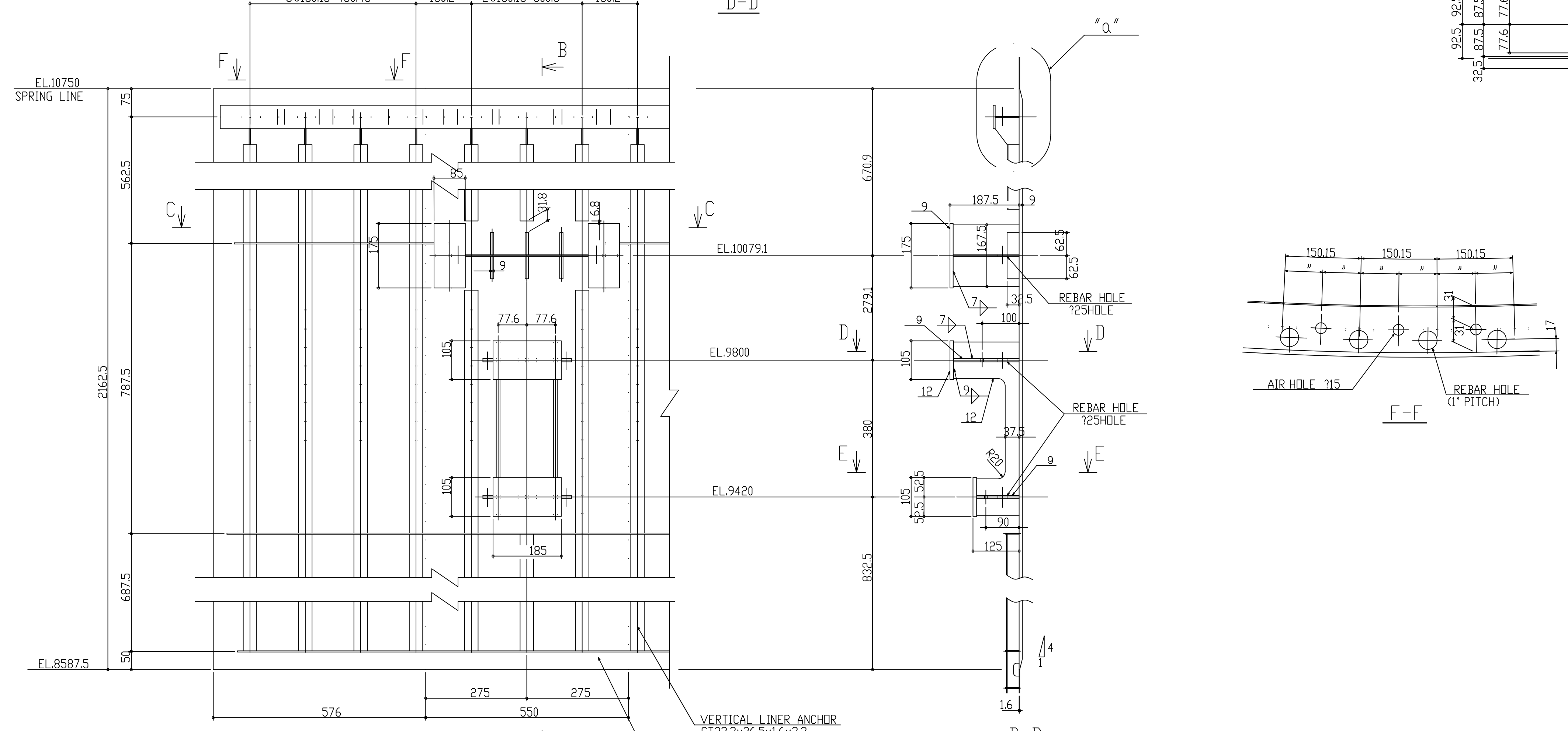
DETAIL "A"
