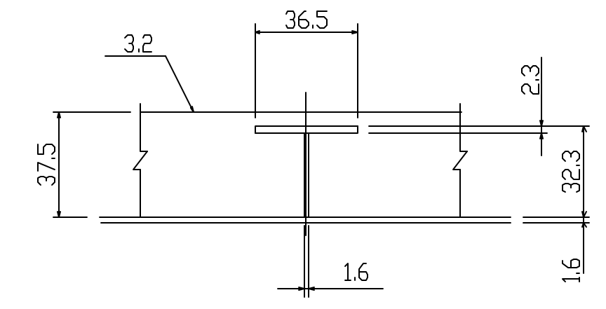
LINER ANCHOR DETAIL
