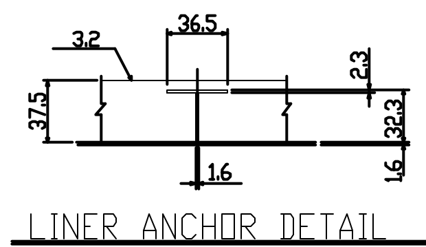
LINER ANCHOR DETAIL
