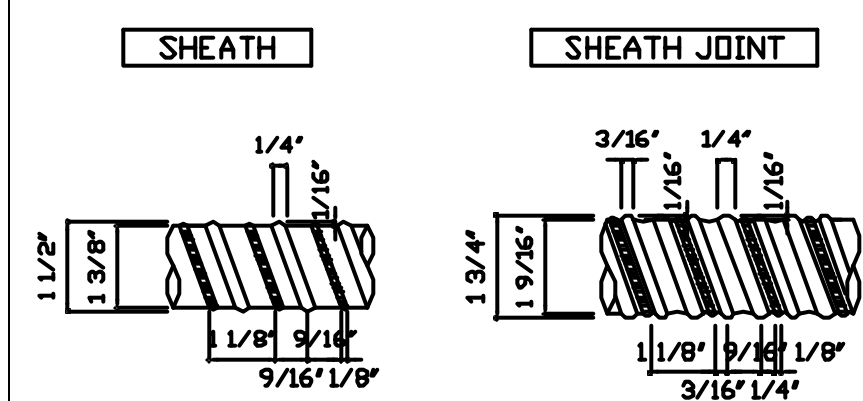
SHEATH DETAIL S=1/2
