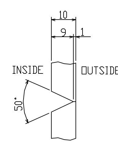
DETAIL "e"
