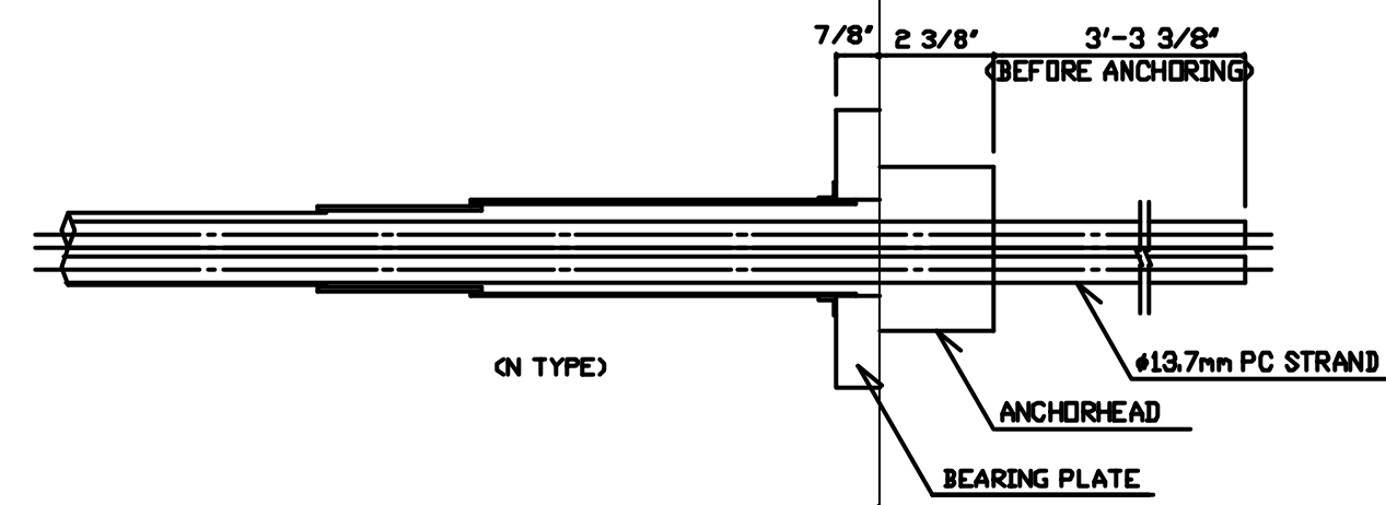
ANCHORED PORTION SECTION S=1/4
