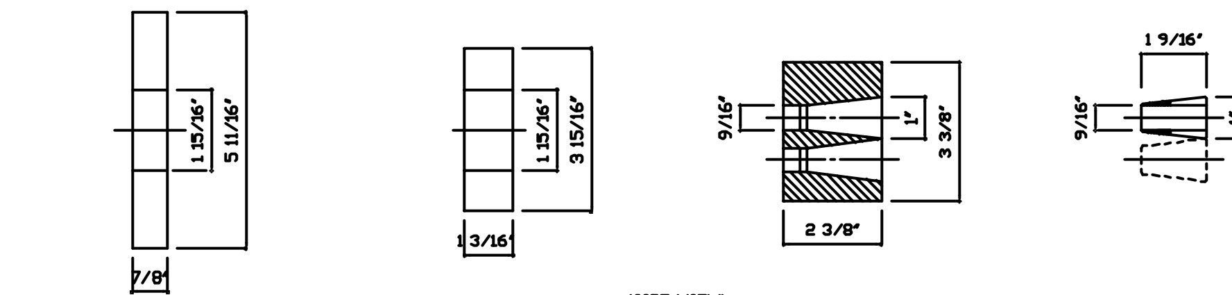
(SIDE VIEW)
