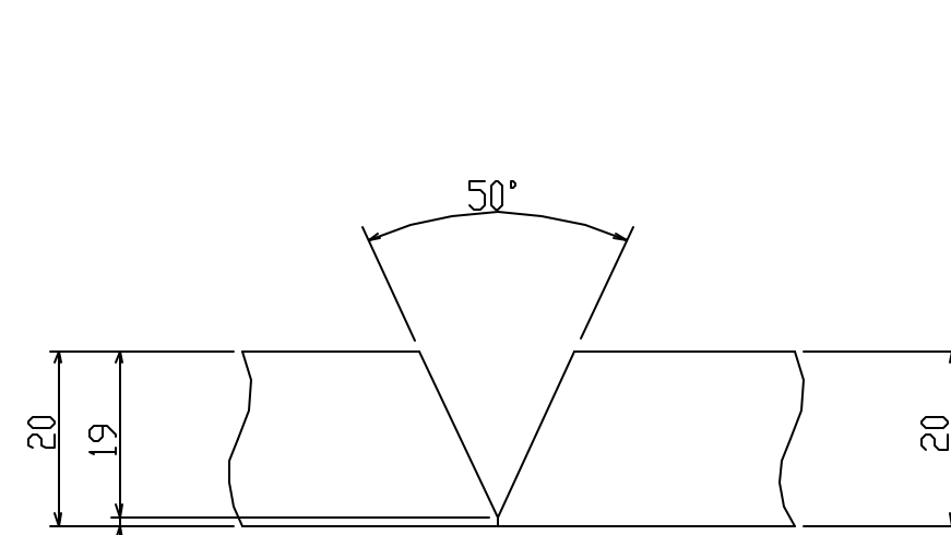
DETAIL "q"
