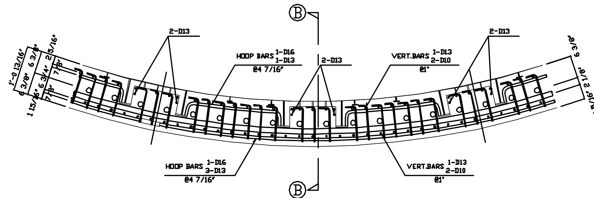
Ⓒ-Ⓒ SECTION DETAILS
