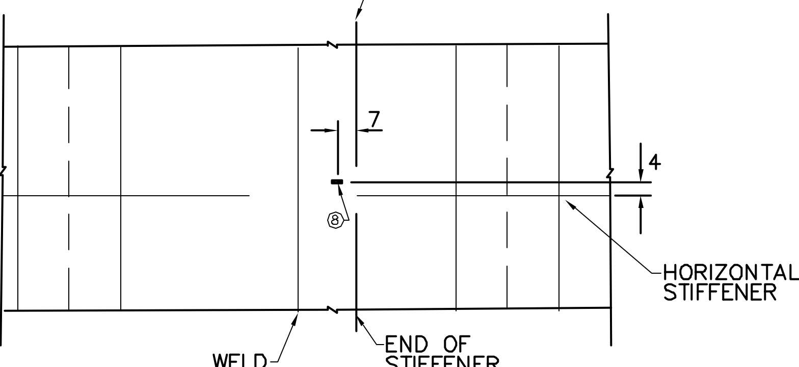
OUTSIDE VIEW
