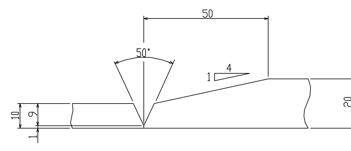
DETAIL "f"
