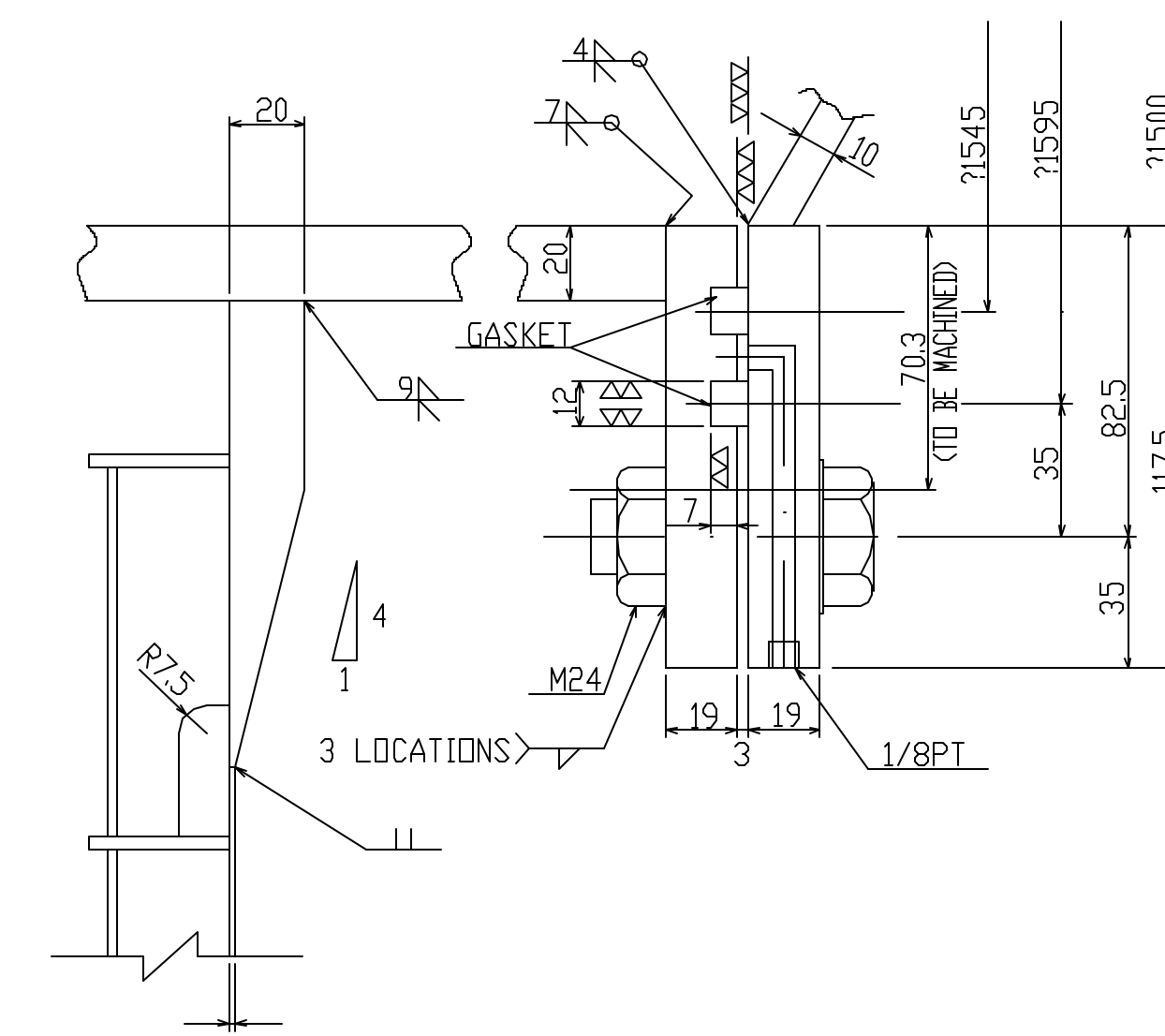
DETAIL "c"
